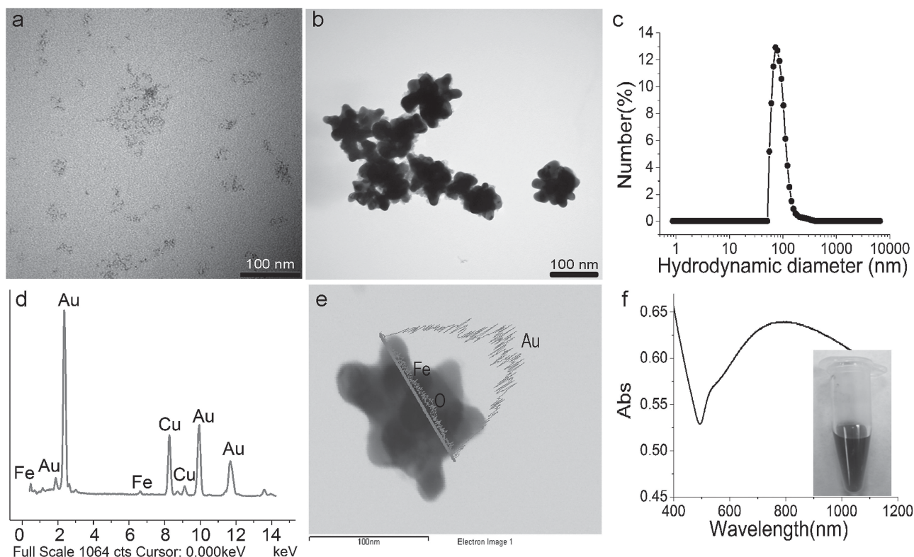
Figure 3. Characterization of \text{Fe}_3\text{O}_4 @Au nanorose. a,b) Transmission electron microscope (TEM) images of a) dextran-coated \text{Fe}_3\text{O}_4 nanoparticles and b) nanoroses. Scale bar = 100 nm. c) Hydrodynamic diameter of nanoroses determined by dynamic light scattering (DLS) in Tris-HCl buffer (pH 7.5). d,e) Energy-dispersive spectroscopy (EDS) line scanning coupled with scanning transmission electron microscopy (STEM) from one nanorose. The outer surface line is from Au, and the lines throughout the cluster diameter are from oxygen and iron, respectively. Cu peaks are from TEM sample grid. f) UV-vis-NIR absorption spectra and solution color of nanoroses in Tris-HCl buffer (pH 7.5).
